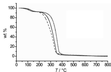
Figure 3. The effect of the anion of basic ionic liquids on the desorption of \text{CO}_2 by TGA: ---- [\text{P}_{66614}][\text{Im}] , — [\text{P}_{66614}][\text{Ind}] , ..... [\text{P}_{66614}][\text{Triz}] .
