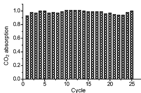
Figure 4. 25 cycles \text{CO}_2 absorption and desorption using [\text{P}_{66614}][\text{Triz}] . \text{CO}_2 absorption was carried out at 25^\circ\text{C} for 20 min, and desorption was performed at 80^\circ\text{C} under \text{N}_2 for 20 min.
