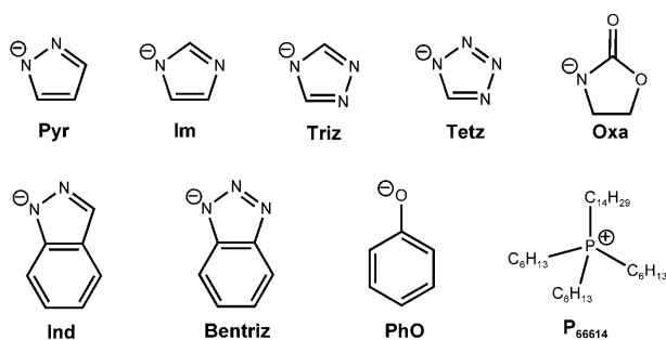
Scheme 1. Structure of anion and cation in tunable basic ILs for CO 2 capture.
