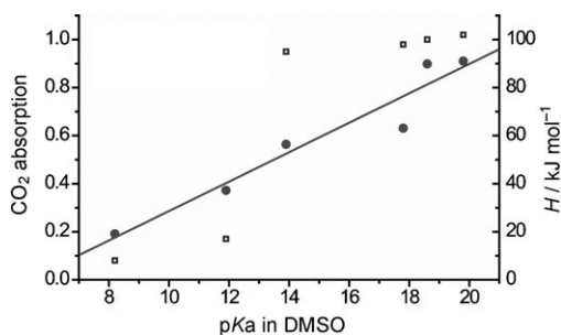
Figure 2. The relationship between \text{CO}_2 absorption capacity ( \square ), absorption enthalpy ( \Delta H , \bullet ), and the \text{p}K_a value of the anion in DMSO. The linear fit for the relationship between \Delta H and \text{p}K_a of the anion in DMSO is shown; R^2 = 0.930 .
