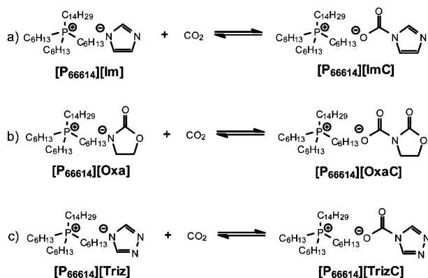
Scheme 2. The \text{CO}_2 absorption mechanism by typical basic ionic liquids.
